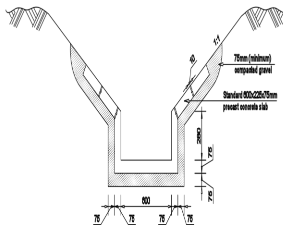
Invert block drain (Type 'B') with two side slabs Scale 1:20
