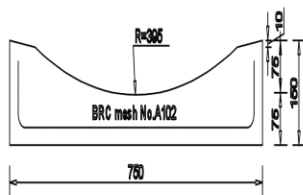
Shallow invert block drain Scale 1:10
