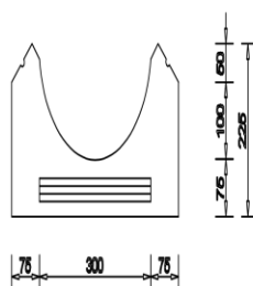
Precast invert block drain (Type 'A') Scale 1:10
