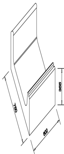
Isometric view of invert block drain Type 'B' Scale 1:20
