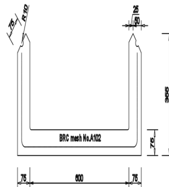
750x355mm invert block drain (Type 'B') Scale 1:10
