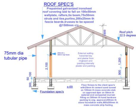
S-Elevation
